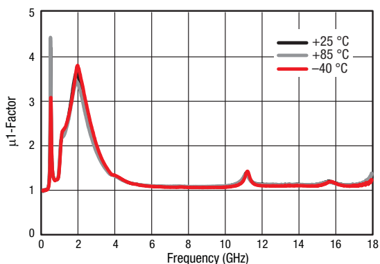
Figure 19. Stability Factor ( \mu_1 ) vs Frequency Over Temperature @ 5 V
