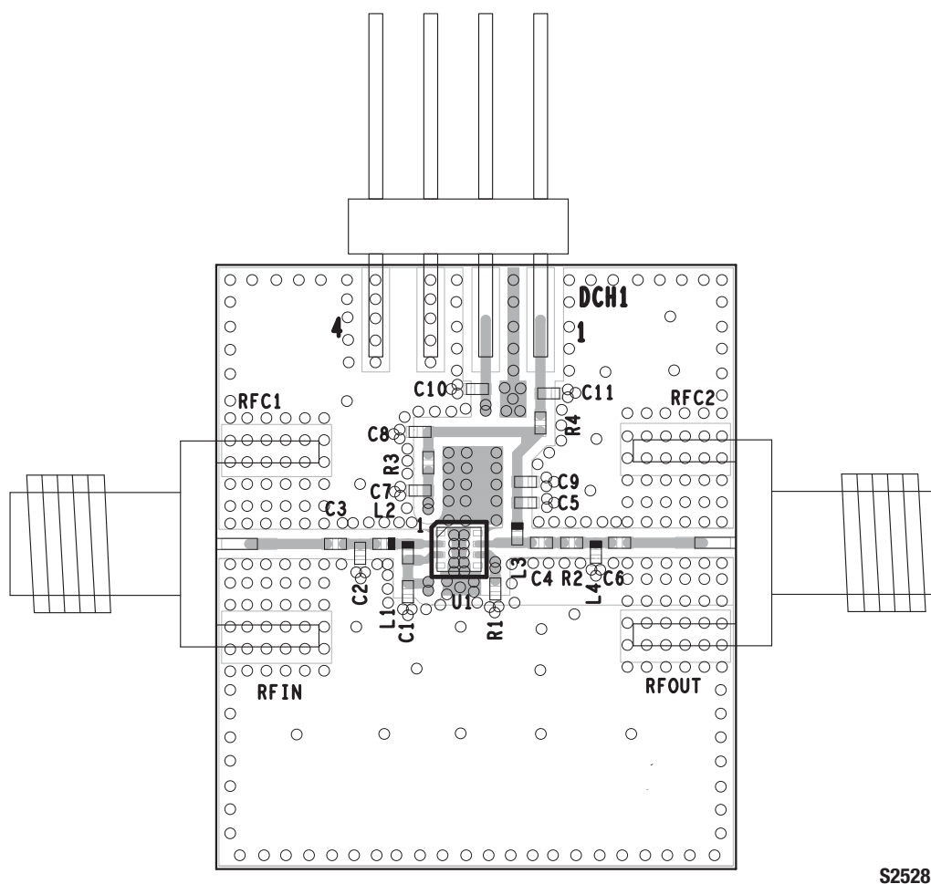
Figure 21. SKY67022-396LF Evaluation Board Assembly Diagram
