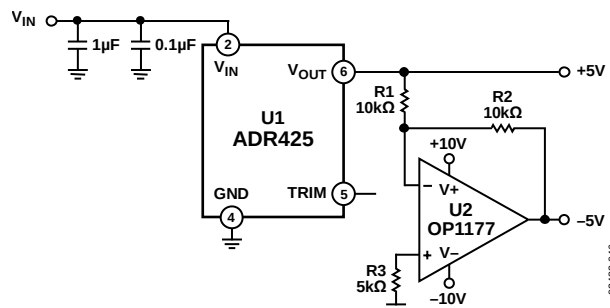
Figure 44. +5 V and -5 V Reference Using ADR425
