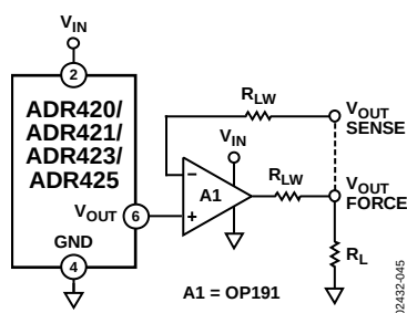
Figure 43. Advantage of Kelvin Connection
