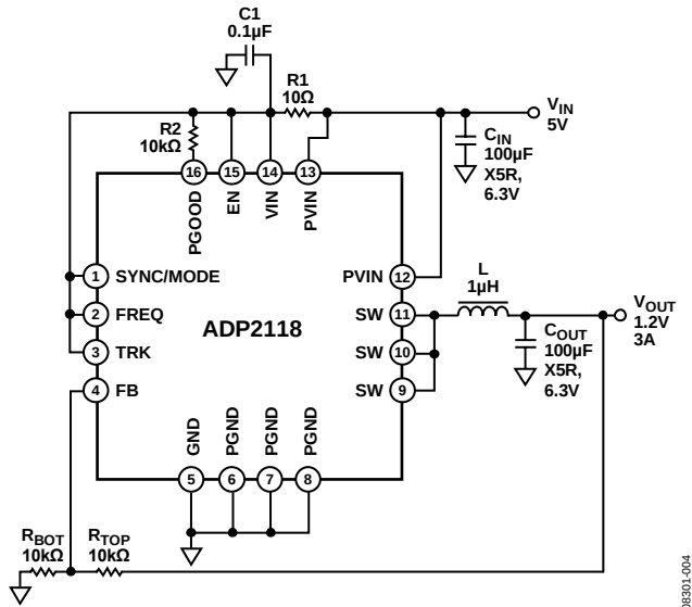
Figure 41. Application Circuit
