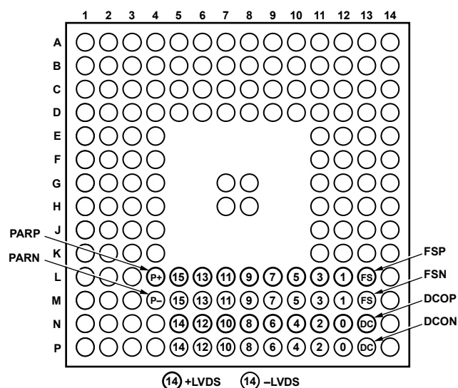
Figure 7. LVDS Mode Data Input Pins (Top View)
