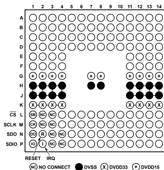
Figure 6. Digital Supply and SPI Pins (Top View)
