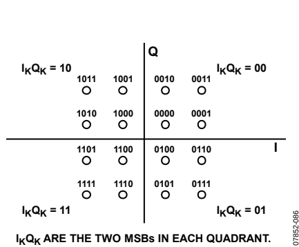
Figure 121. DVB-C 16-QAM Constellation
