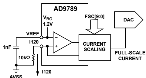
Figure 108. Voltage Reference Circuit
