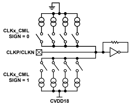
Figure 115. Clock Common-Mode Control
