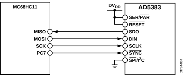
Figure 34. AD5383-to-MC68HC11 Interface
