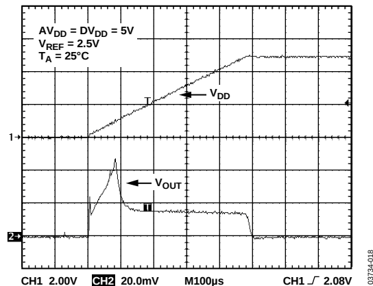
Figure 18. Power-Up Transient
