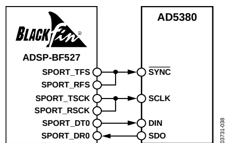
Figure 38. AD5380-to-ADSP-BF527 Interface
