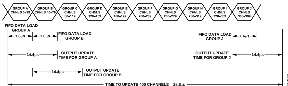
Figure 49. Using FIFO Mode 400 Channels Updated in Under 30 \mu\text{s}
