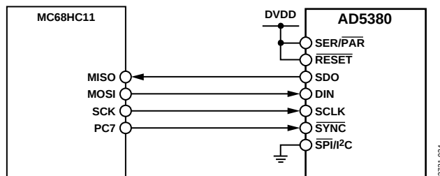
Figure 34. AD5380-to-MC68HC11 Interface
