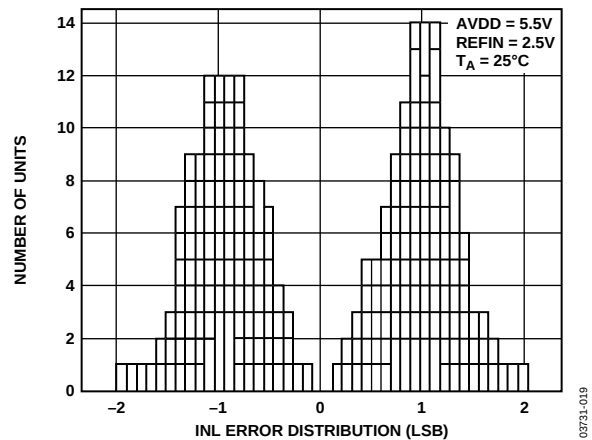
Figure 19. INL Distribution
