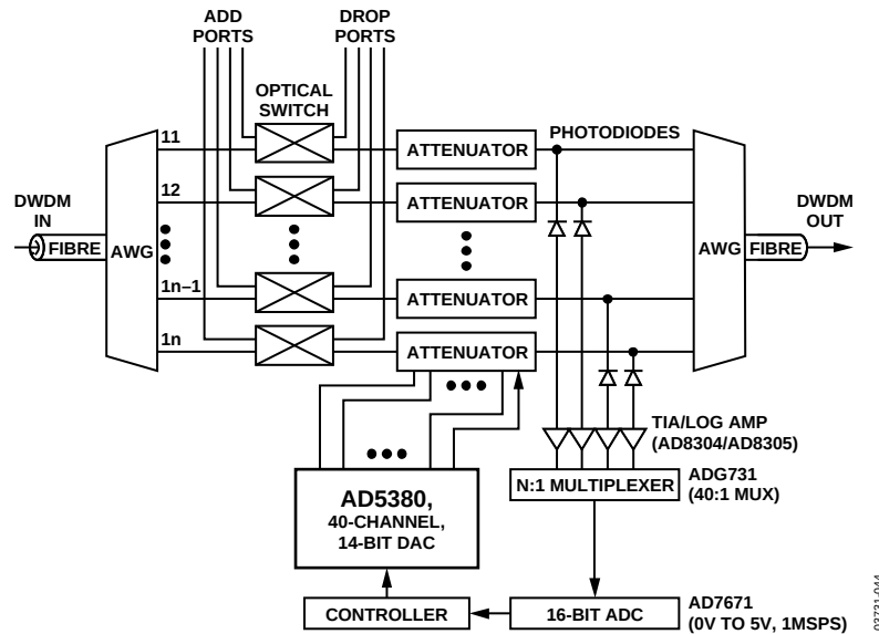
Figure 48. OADM Using the AD5380 as Part of an Optical Attenuator
