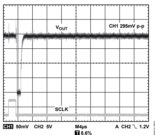
Figure 35. Glitch Upon Entering Power-Down ( 1\text{ k}\Omega to GND) from Zero Scale, No Load
