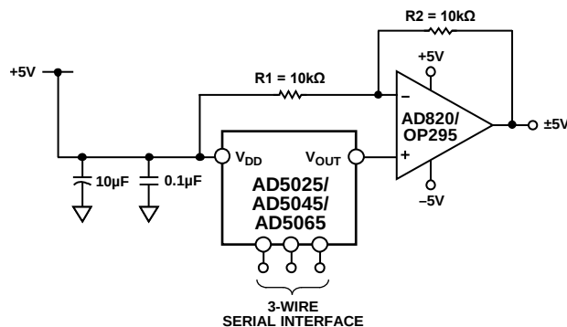
Figure 51. Bipolar Operation with the AD5025/AD5045/AD5065
