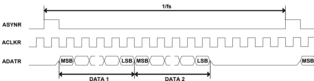
FIGURE 14. ACLMASTER = 0, RM_SYNC = 1
