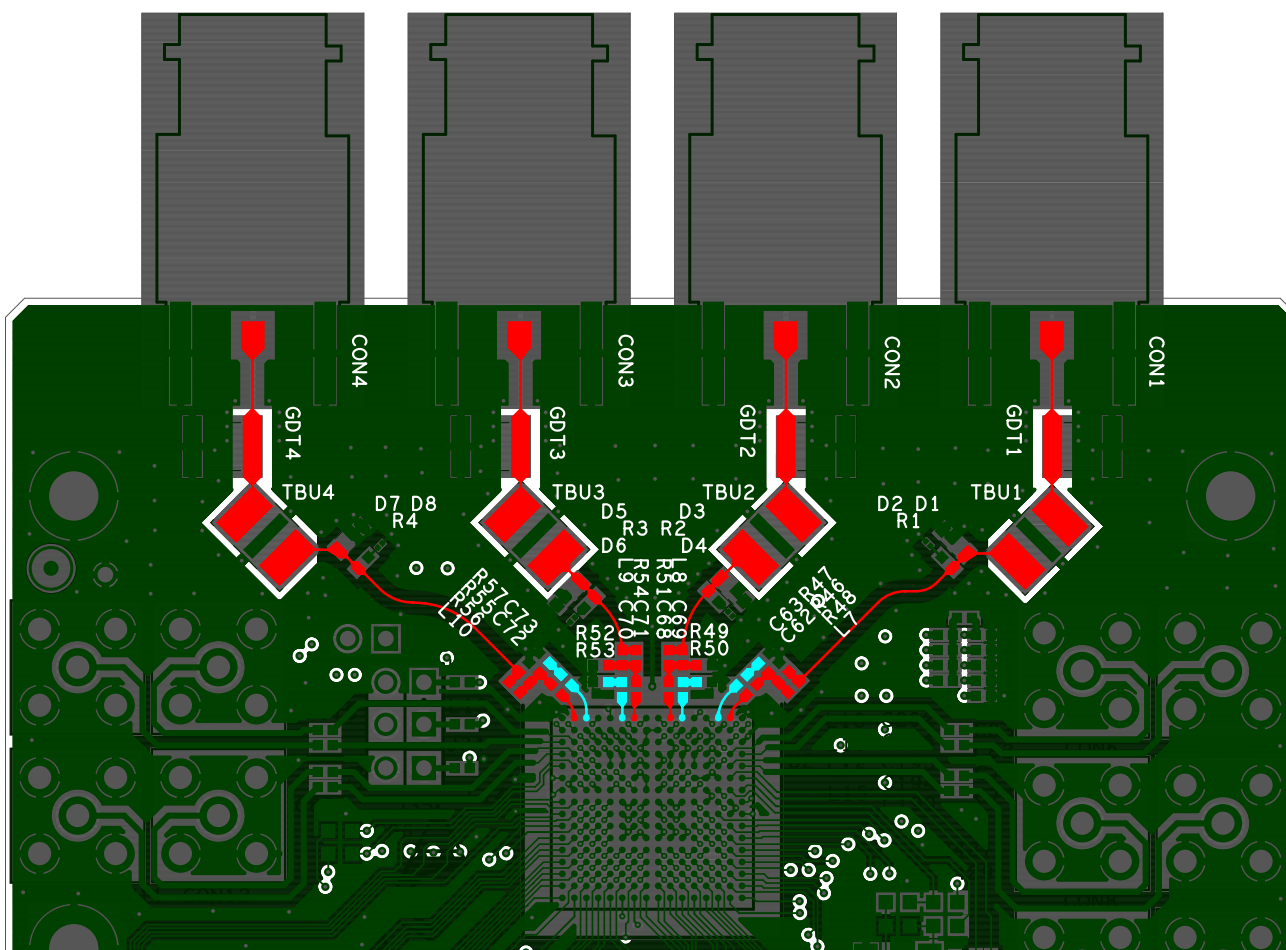
FIGURE 35. SDI1-4 LAYOUT LAYER 1
