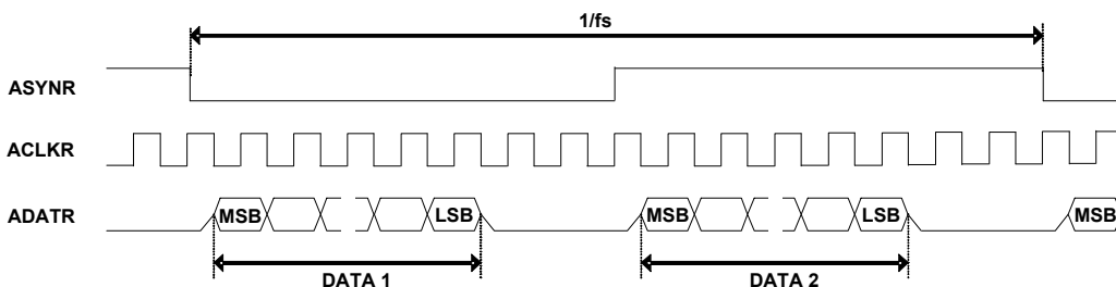
FIGURE 15. ACLMASTER = 0, RM_SYNC = 0, ASYNROEN = 1
