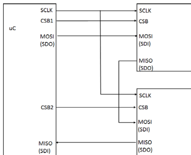
FIGURE 33. INTERFACING TO MULTIPLE SPI SLAVES
