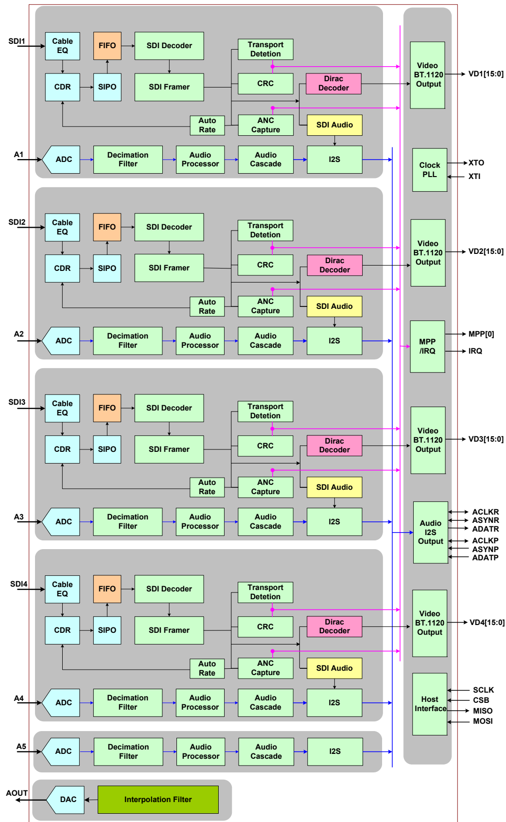
FIGURE 2. BLOCK DIAGRAM
