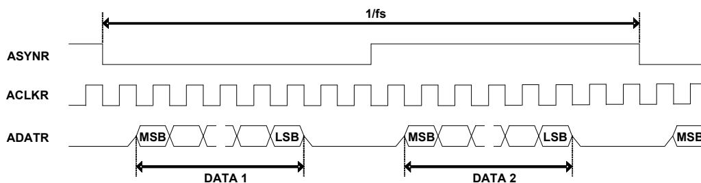
FIGURE 13. ACLMASTER = 0, RM_SYNC = 0
