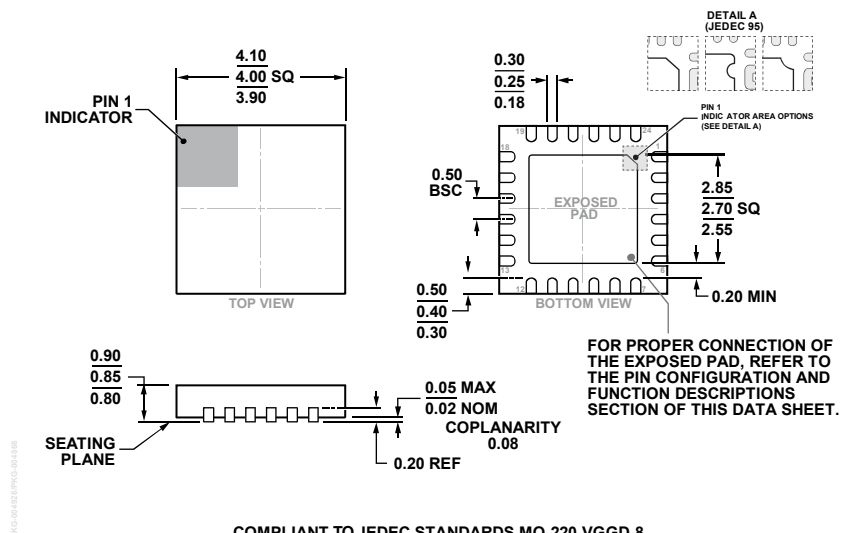
Figure 35. 24-Lead Lead Frame Chip Scale Package [LFCSP] 4 mm × 4 mm Body and 0.85 mm Package Height (CP-24-16)
