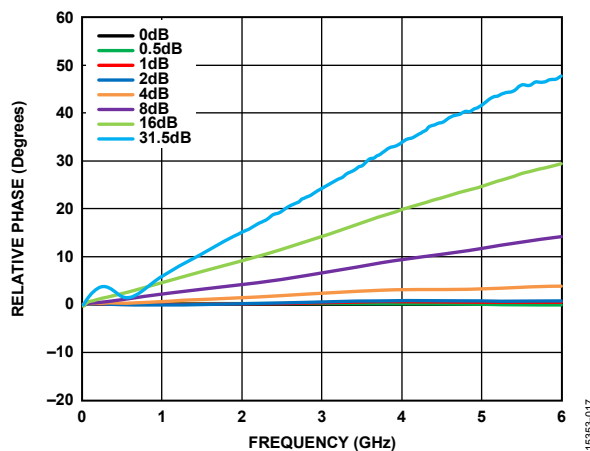
Figure 17. Relative Phase vs. Frequency over Major Attenuation States
