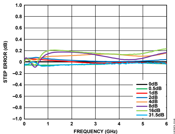
Figure 16. Step Error vs. Frequency over Major Attenuation States
