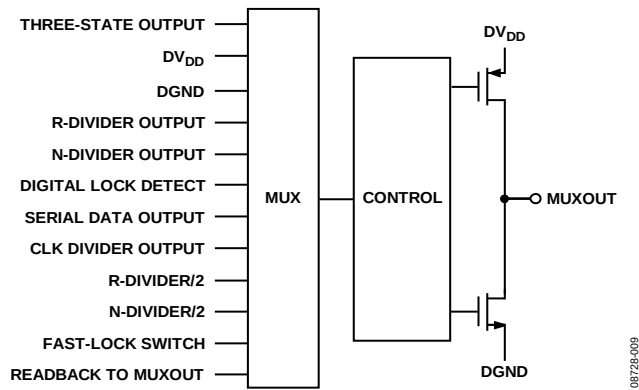
Figure 20. MUXOUT Schematic
