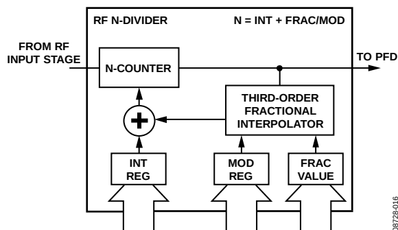
Figure 18. RF N-Divider
