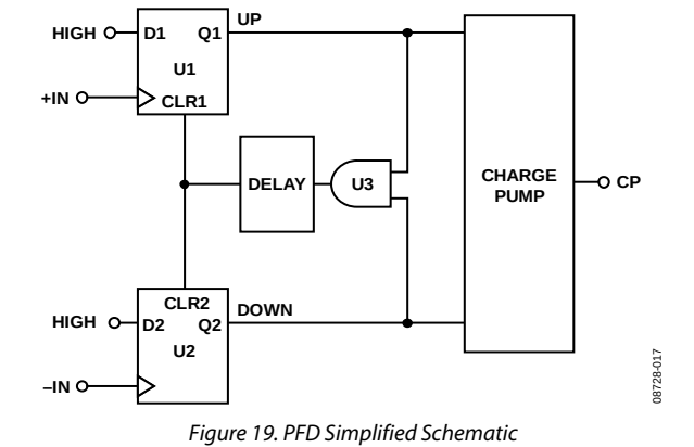
Figure 19. PFD Simplified Schematic
