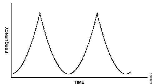
Figure 40. Parabolic Ramp
