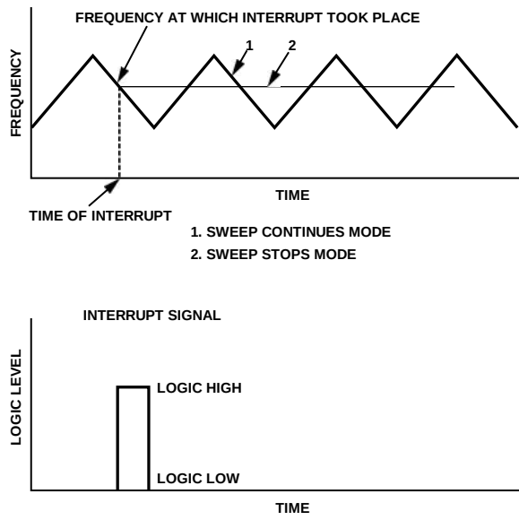
Figure 43. Interrupt and Frequency Readback
