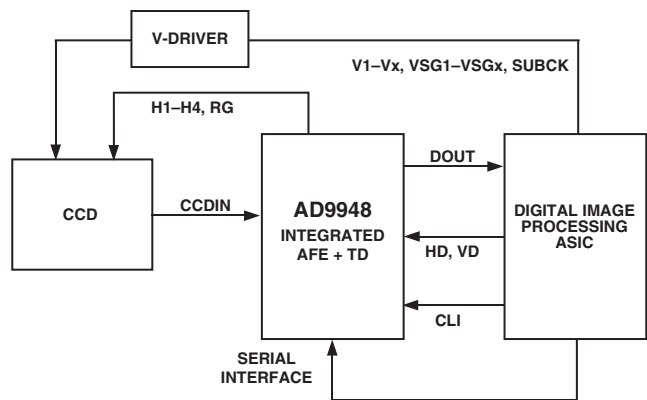
Figure 1. Typical Application
