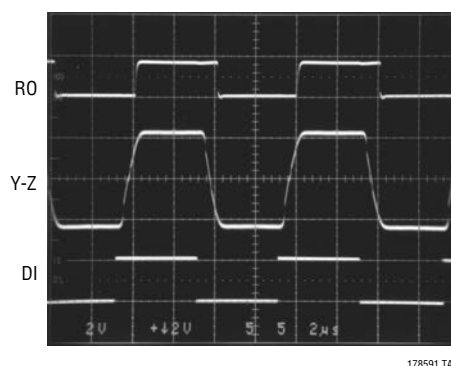
Normal Operation Waveforms at 250kbaud
