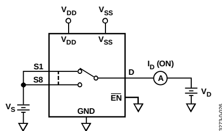
Figure 24. I_D (ON)
