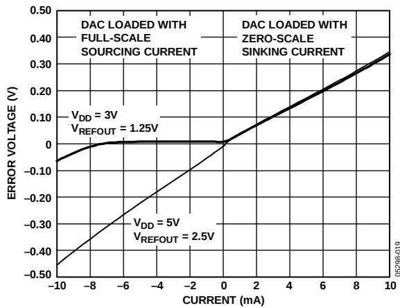
Figure 18. Headroom at Rails vs. Source and Sink
