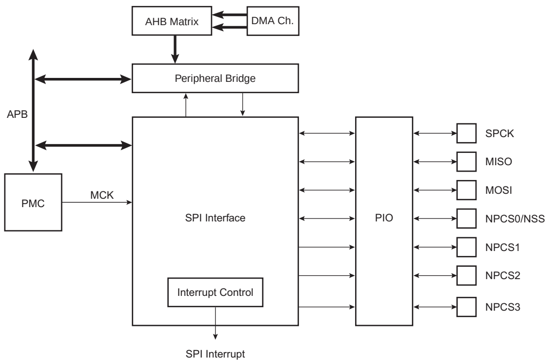
Figure 32-1. Block Diagram
