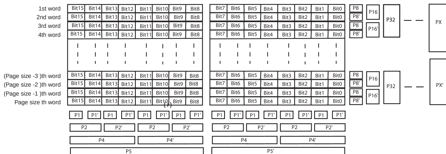
Figure 25-40. Parity Generation for 512/1024/2048/4096 16-bit Words
