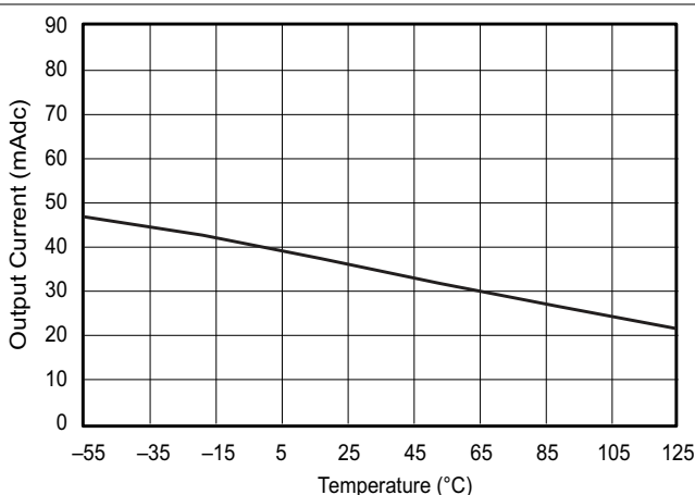
Figure 6-48. Source Current Limiting
