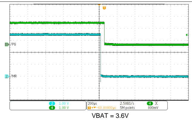
Figure 73. \overline{\text{PG}} \overline{\text{MR}} Level Shift Function - \overline{\text{MR}} Falling
