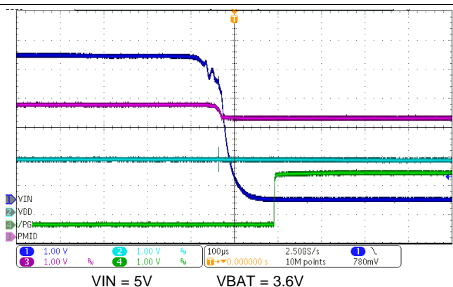
Figure 71. \overline{\text{PG}} Power Good Function - IN Supply Removal
