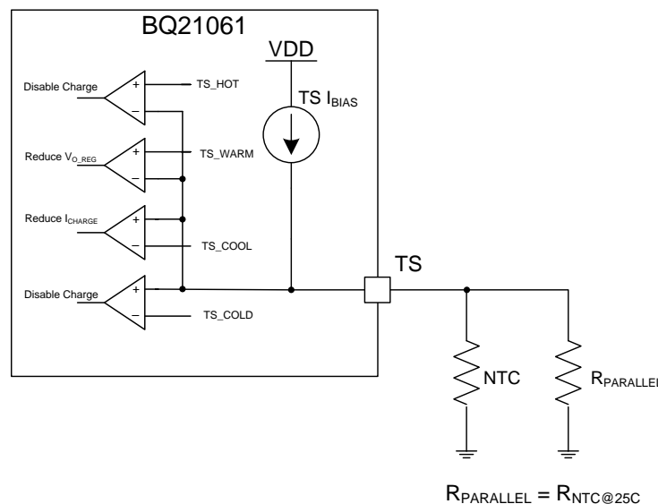
Figure 23. TS Bias Functional Diagram
