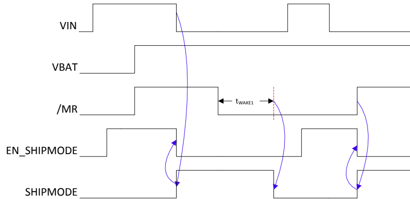
Figure 28. Ship Mode Entry Based On EN_SHIPMODE bit
