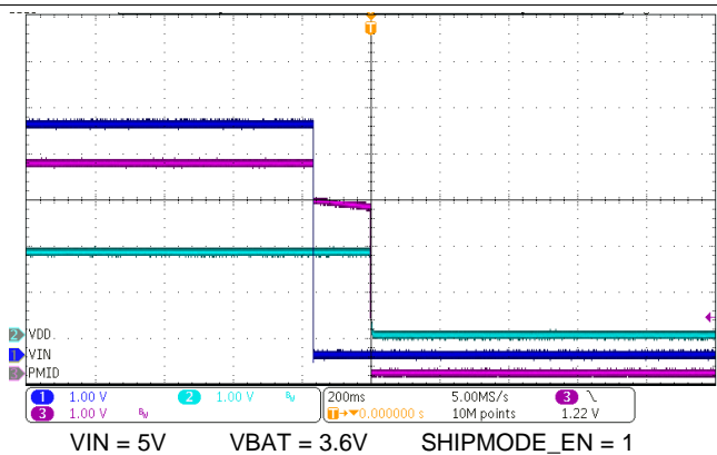
Figure 69. Ship Mode Entry on IN Supply Removal
